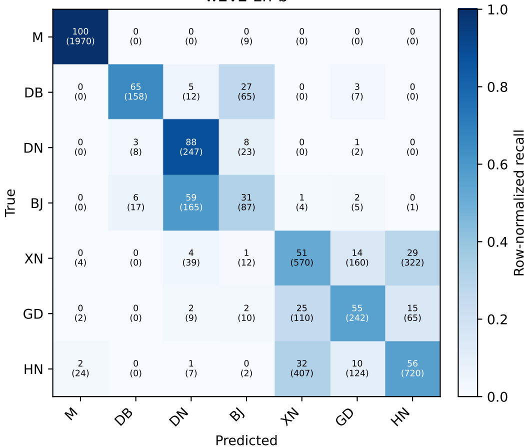
w2v2-zh-b
