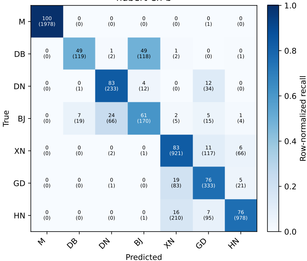
hubert-en-b
