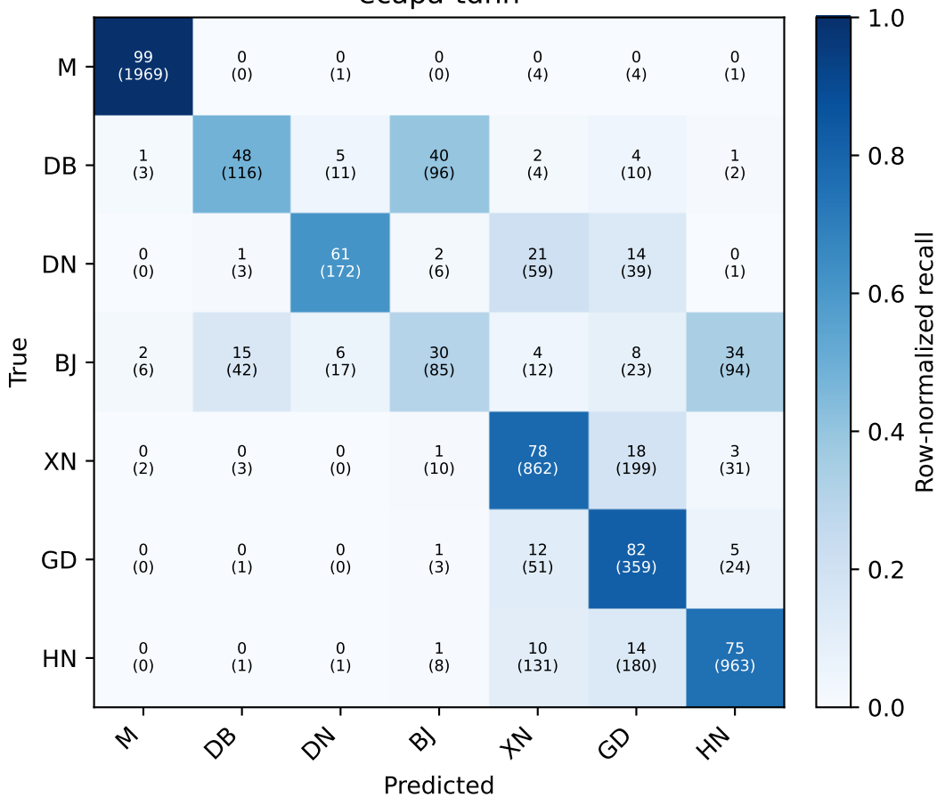
ecapa-tdnn
