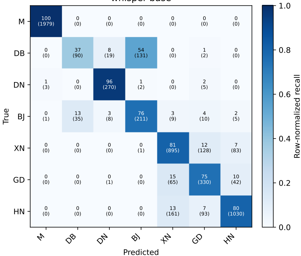
whisper-base
