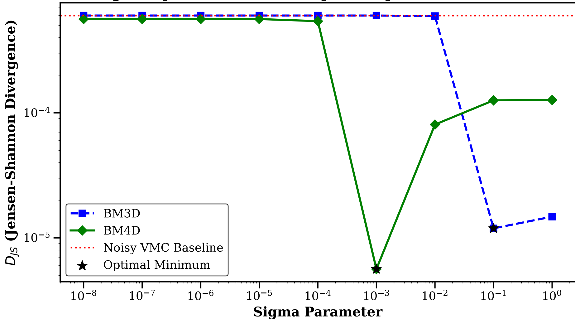
Sigma Optimization Landscape (Sample Size: 10321920)
