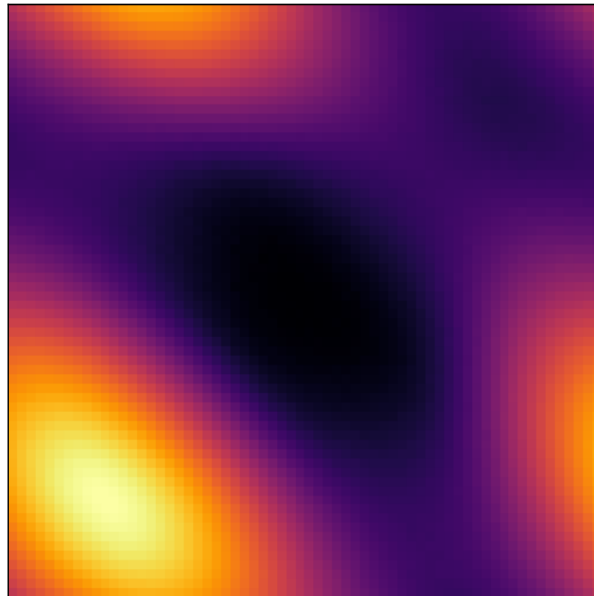
VMC Reference
