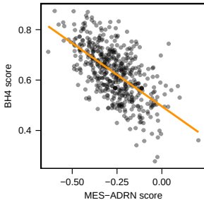
BH4_recycling_regeneration
