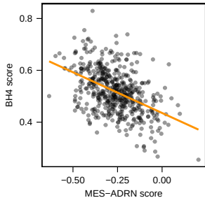
BH4_denovo_synthesis_recycling_regeneration
