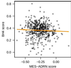
BH4_denovo_synthesis
