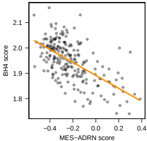
BH4_recycling_regeneration
