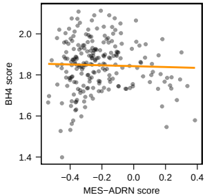
BH4_denovo_synthesis
