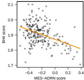
BH4_denovo_synthesis_recycling_regeneration
