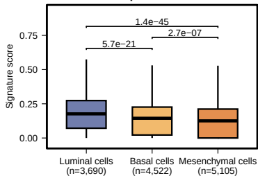
BH4_recycling_regeneration KW p = 6.15e-46
