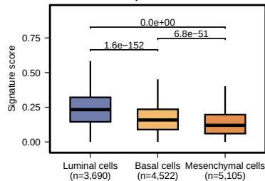
BH4_denovo_synthesis_recycling_regeneration KW p = 0.00e+00
