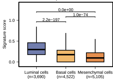
BH4_denovo_synthesis KW p = 0.00e+00
