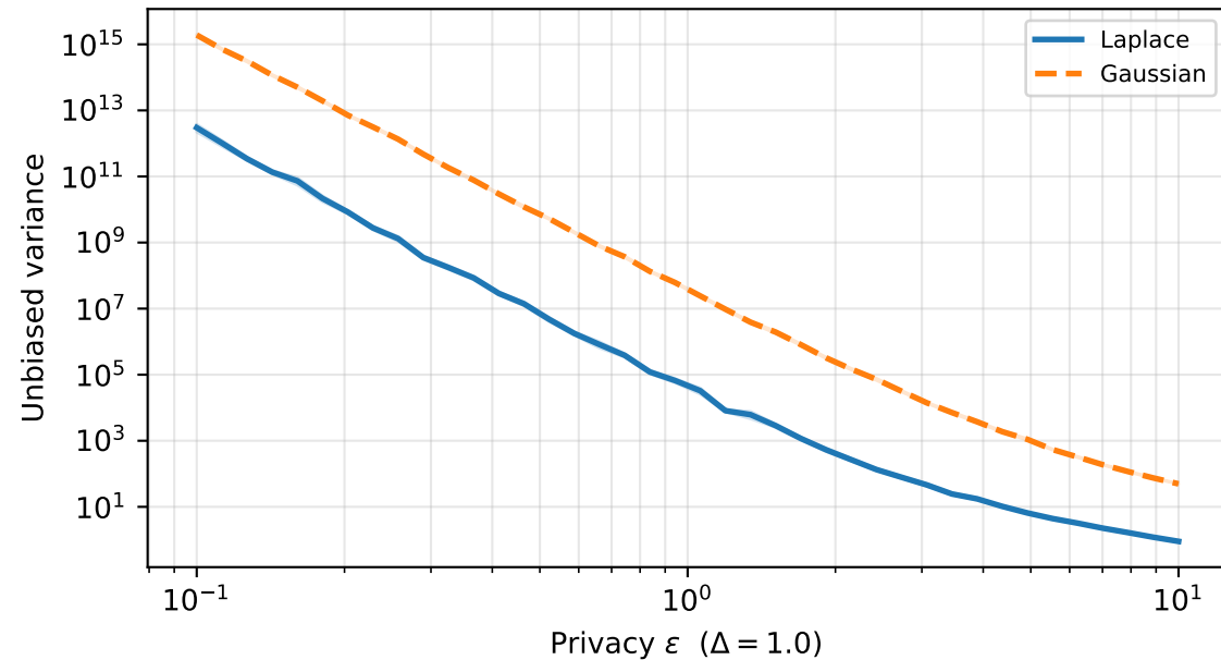
Unbiased variance
