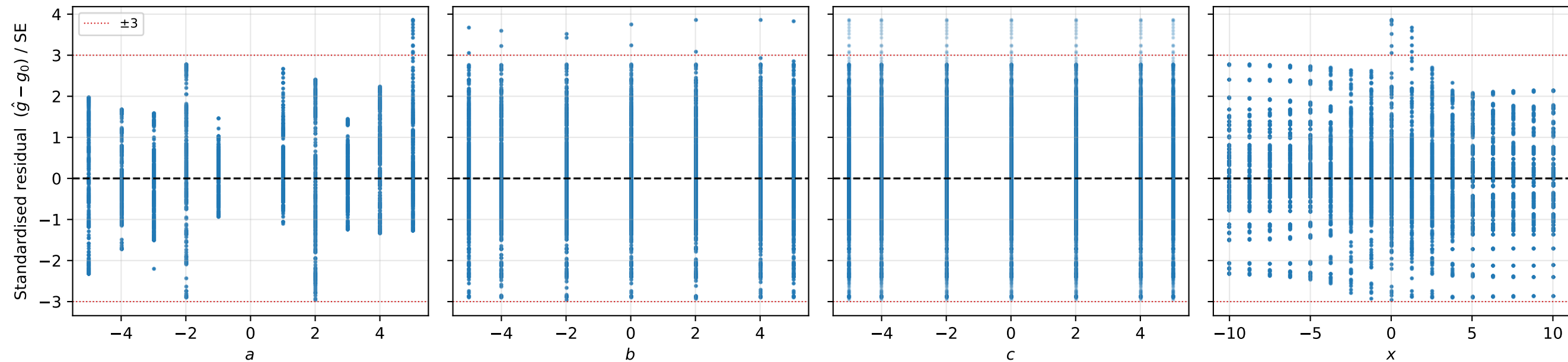
Exp. Q — Standardised MSE-gap residuals over quadratics (99.8% within \pm 3 SE, max = 3.84 SE, \Delta = 1.0 ) No tilt in b , c , x panels \Rightarrow MSE-gap independent of b , c , x (confirms theory -4a^2s^4 )
