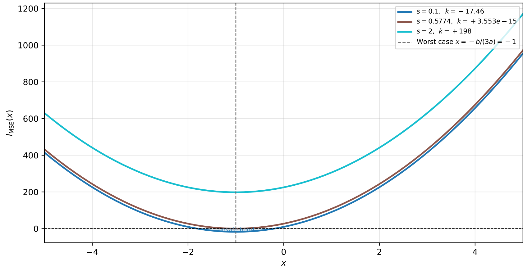
Gap inner polynomial f(q) = 1q^3 + 3q^2 : vertical translations across noise scales
