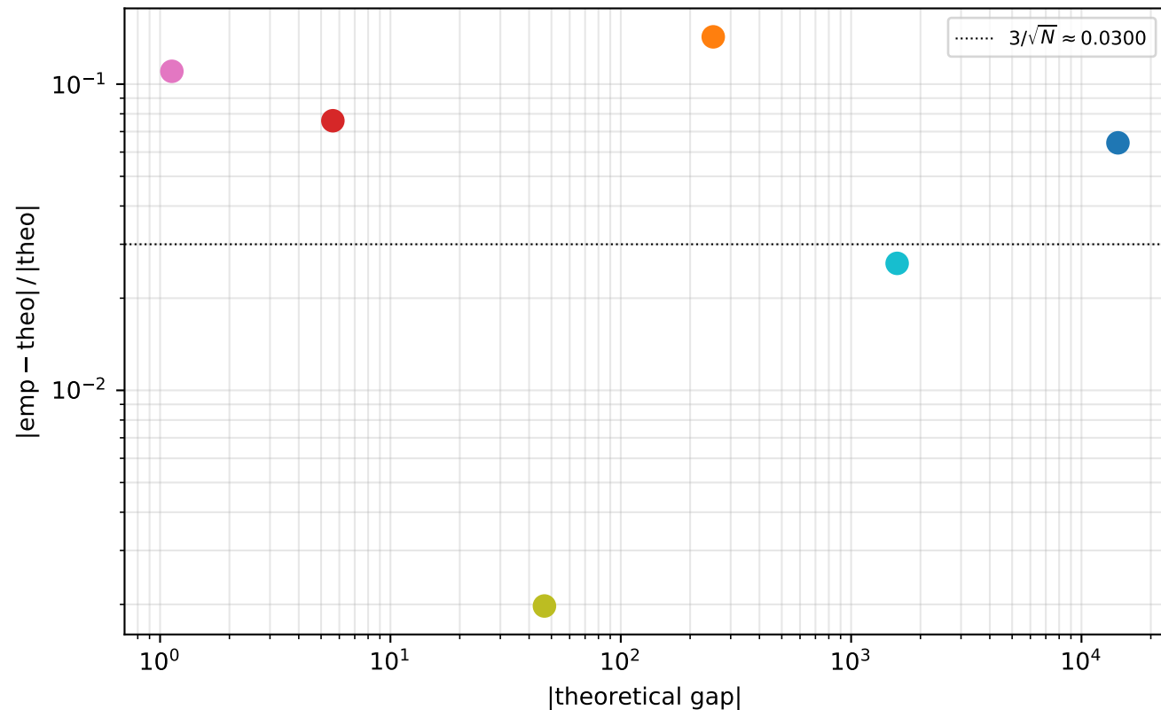
Relative error vs gap magnitude
