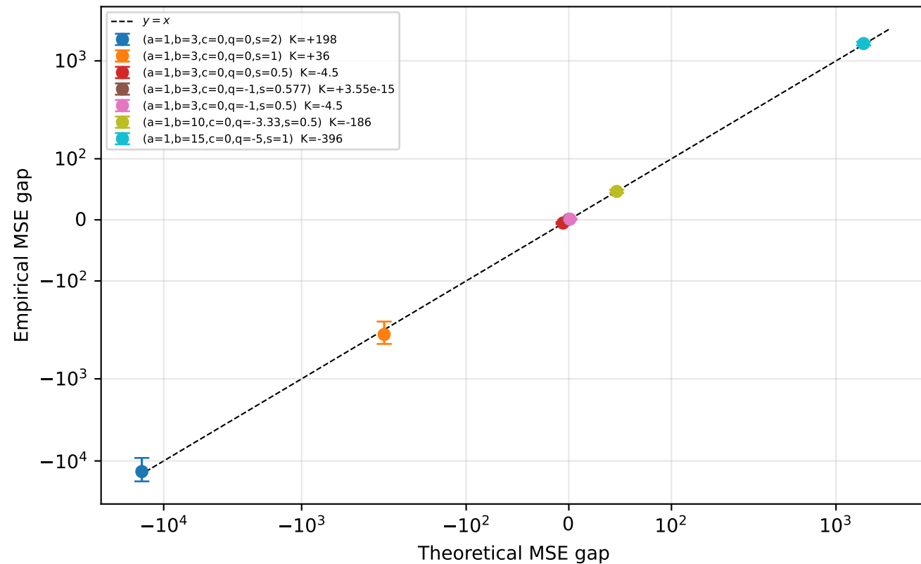
MC validation: empirical vs theoretical (N=10,000)
