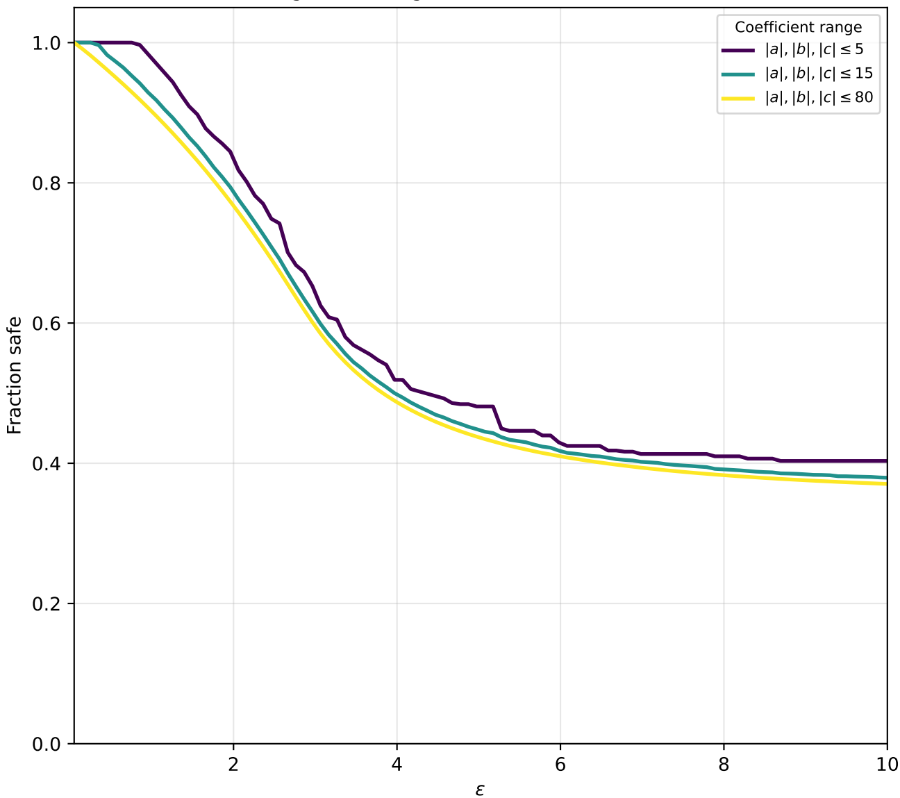
Fraction of integer (a, b, c) grid with K = 54a^2s^2 + 6ac - 2b^2 \geq 0 vs \varepsilon
