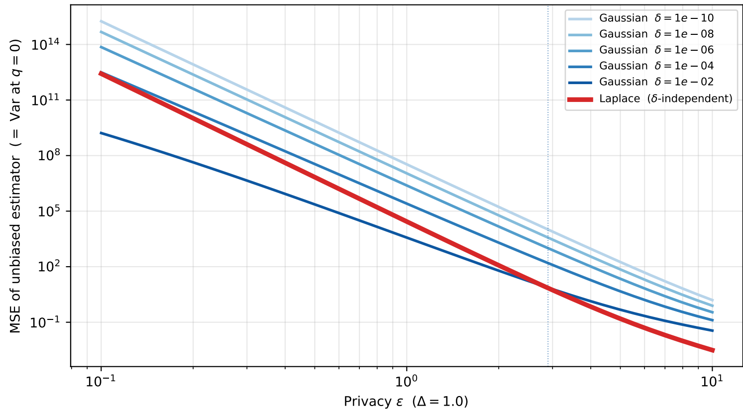
Exp. G (Part A) — Matched-privacy Laplace vs Gaussian, varying \delta q = 0 , \Delta = 1.0 (closed form, no Monte Carlo)
