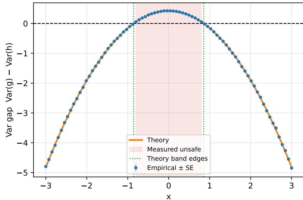
Variance gap
