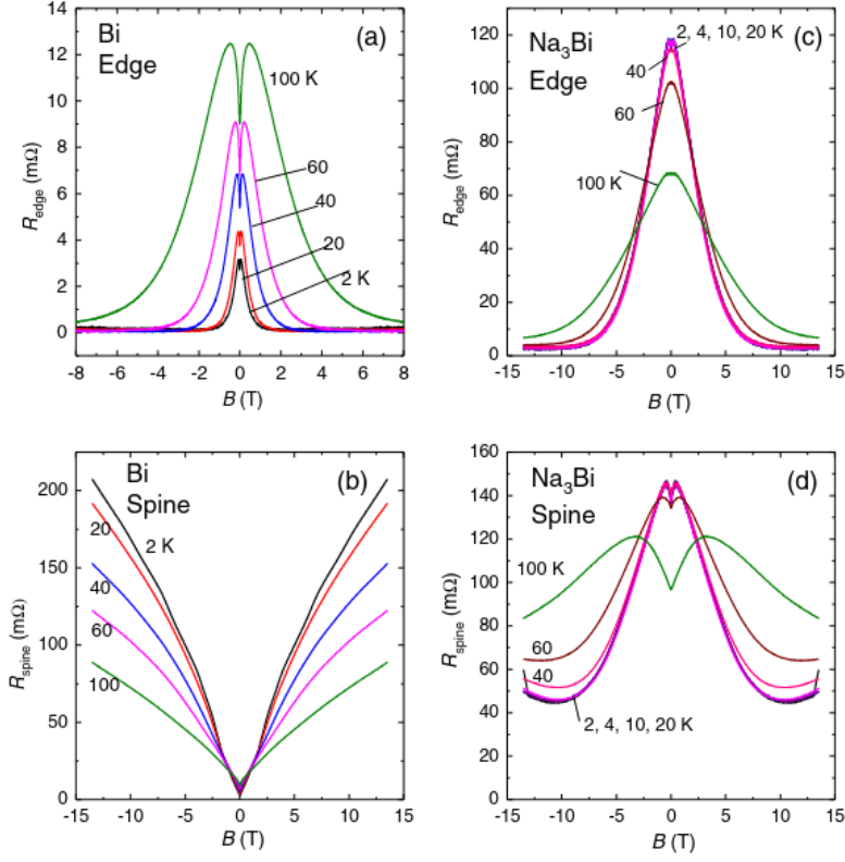
Figure 1. [53] Squeeze test results in pure Bi and \text{Na}_3\text{Bi} at various temperatures shown on the left and right respectively.
