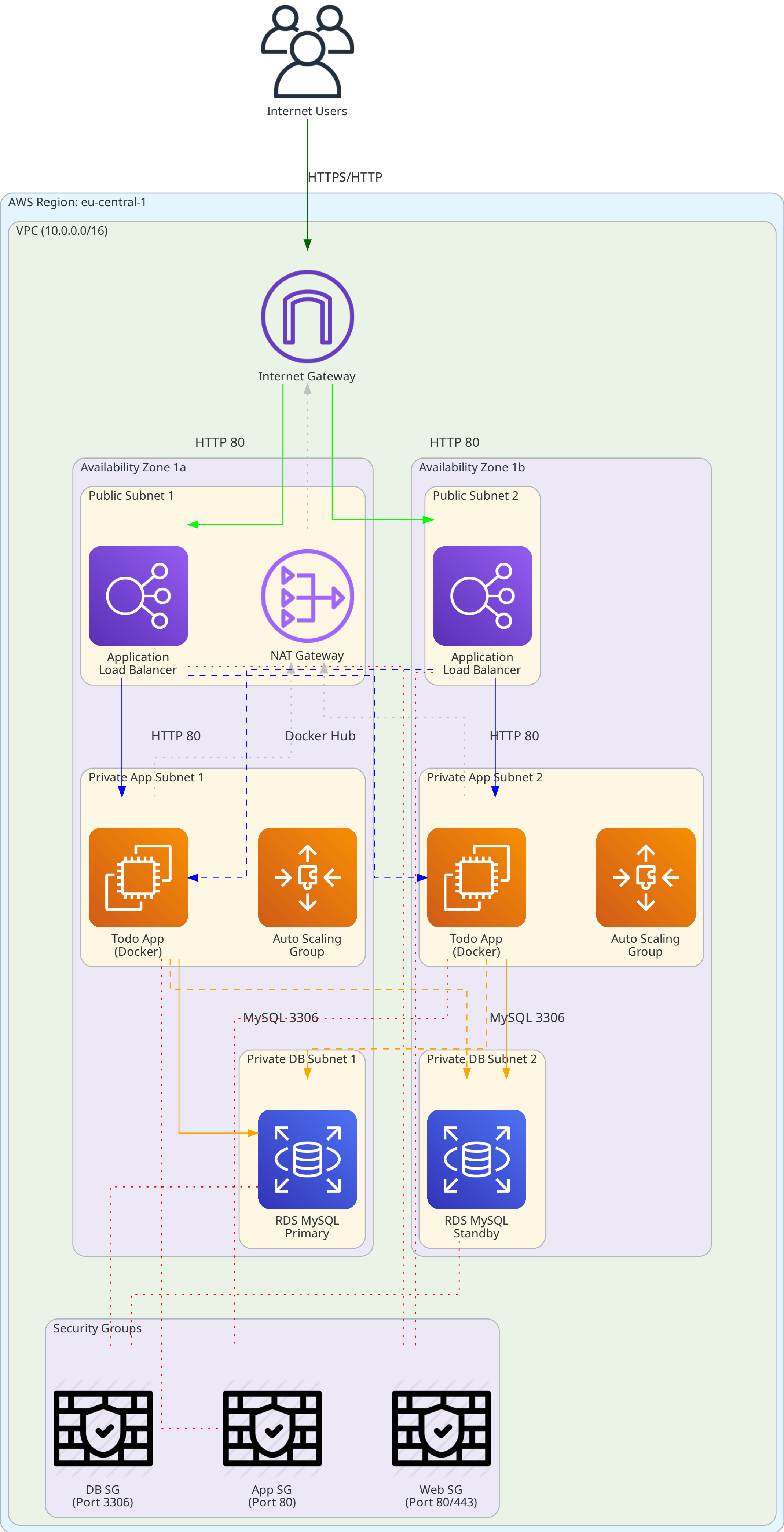
3-Tier AWS Architecture - IaC Project
