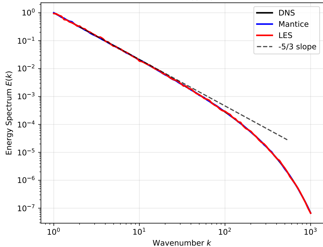
Turbulence Energy Spectrum
