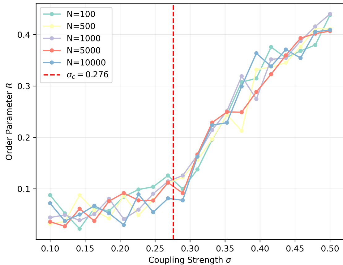
Phase Transition
