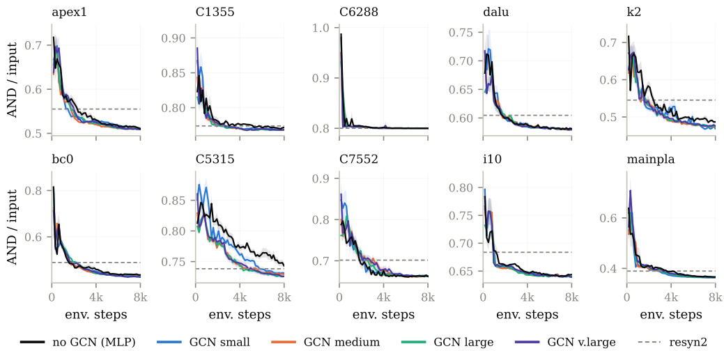
Figure 5: Per-benchmark learning curves for the runs aggregated in figure 2(a). Dashed line: resyn2.
