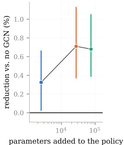
(c) improvement vs. encoder size
