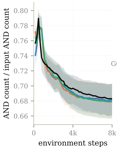
(a) mean over 80 benchmarks
