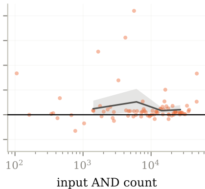
GCN medium
