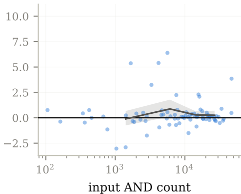
GCN small
