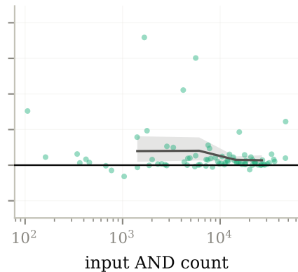
GCN large
