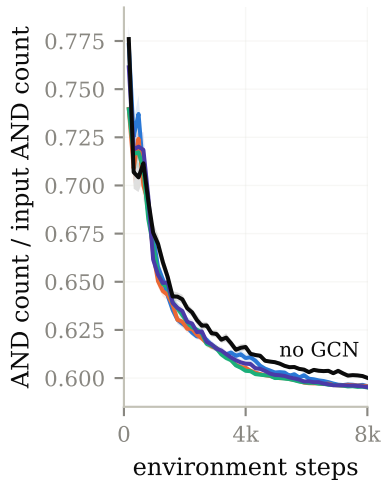
(a) mean over 10 benchmarks
