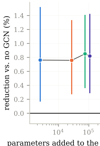
(c) improvement vs. encoder size
