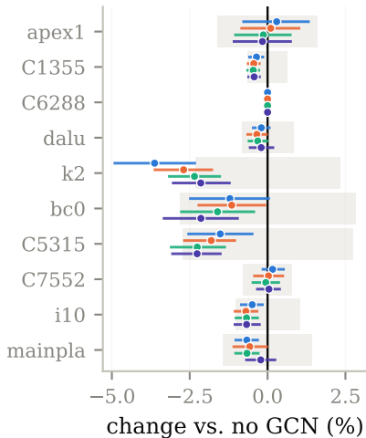
(b) effect of the GCN
