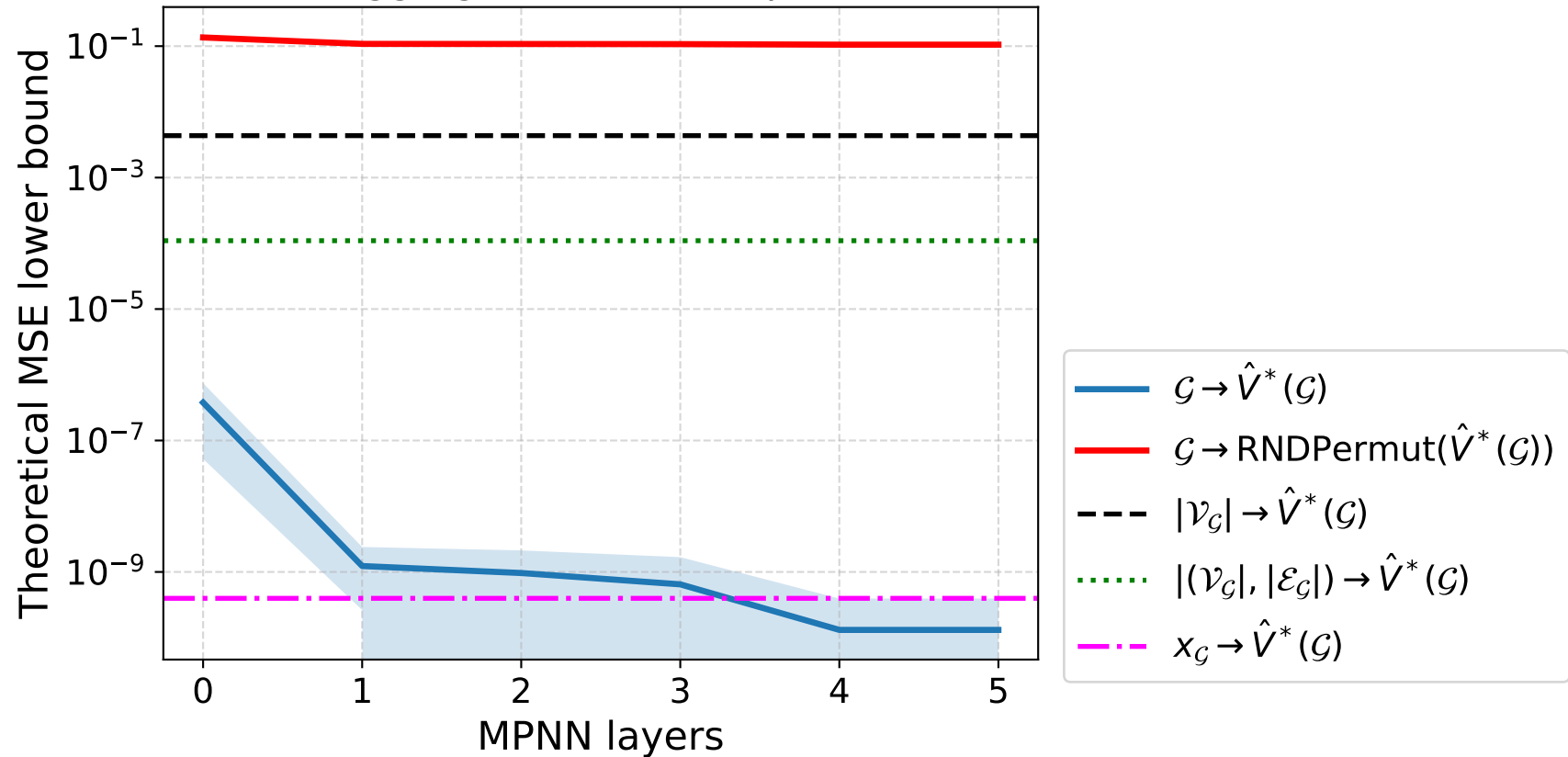
Random aggregation of non-equivalent AIGs
