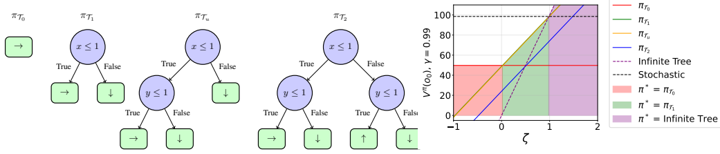
Figure 2: Decision tree policies and their RL objective values (definition 2) as functions of the rewards \zeta in POIBMDPs associated to the grid world MDP (figure 1b). Shaded areas on the right plot indicate which deterministic memoryless policy is optimal depending on \zeta . Recall that \zeta can be seen as a reward that encourages the deterministic memoryless policy to take information-gathering actions, i.e. the reward that trades off interpretability of the corresponding decision tree and its cumulative reward.
