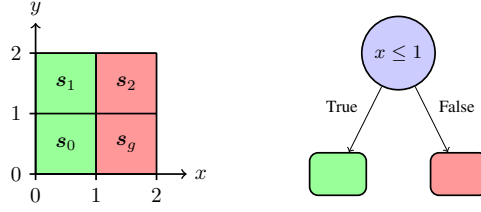
Figure 5: In this MDP, there are four data to which to assign either a green or red label. On the right, there is the unique optimal depth-1 tree for this particular MDP. This depth-1 tree also maximizes the accuracy on the corresponding classification task.
