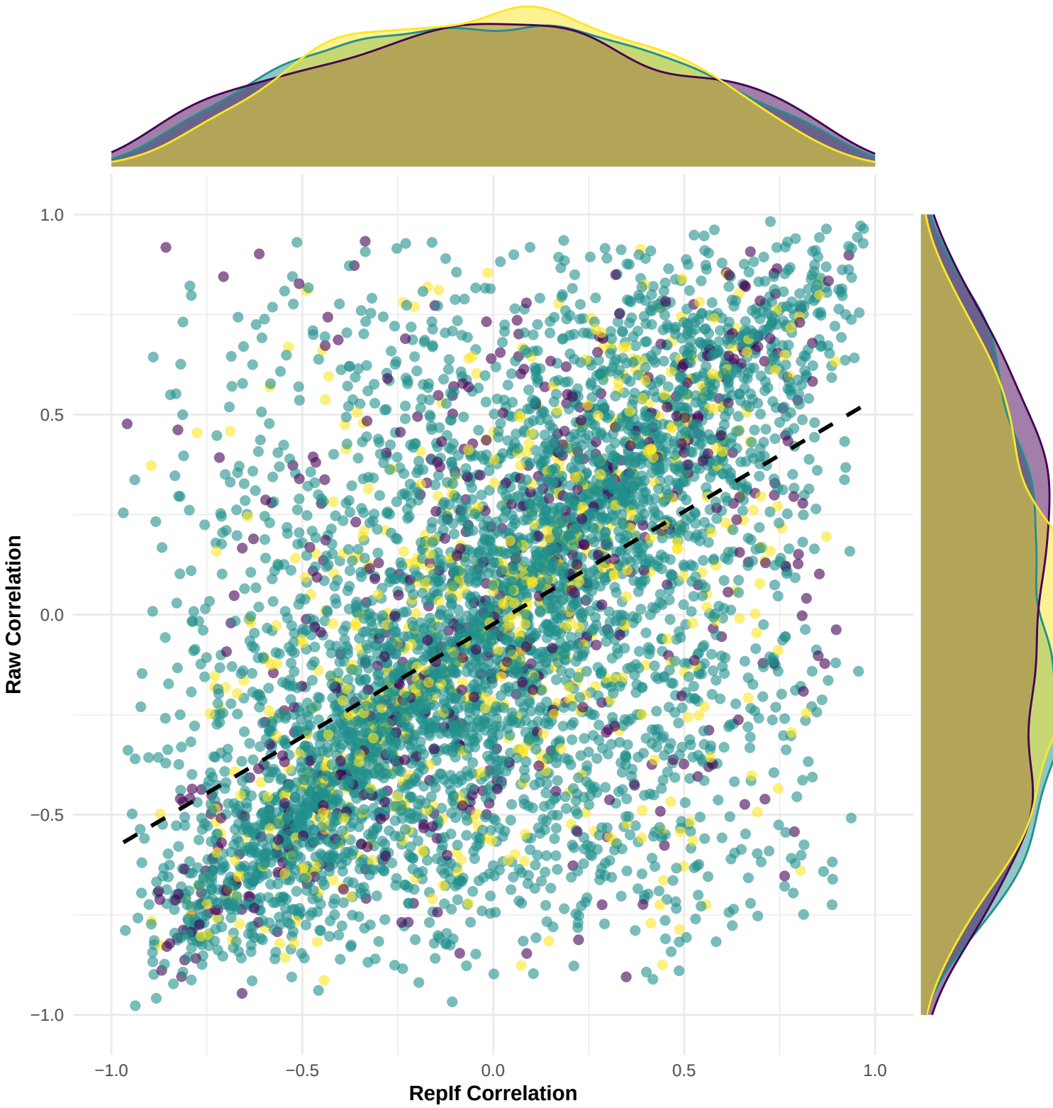
MidBrain – Methylation–Expression Correlations
