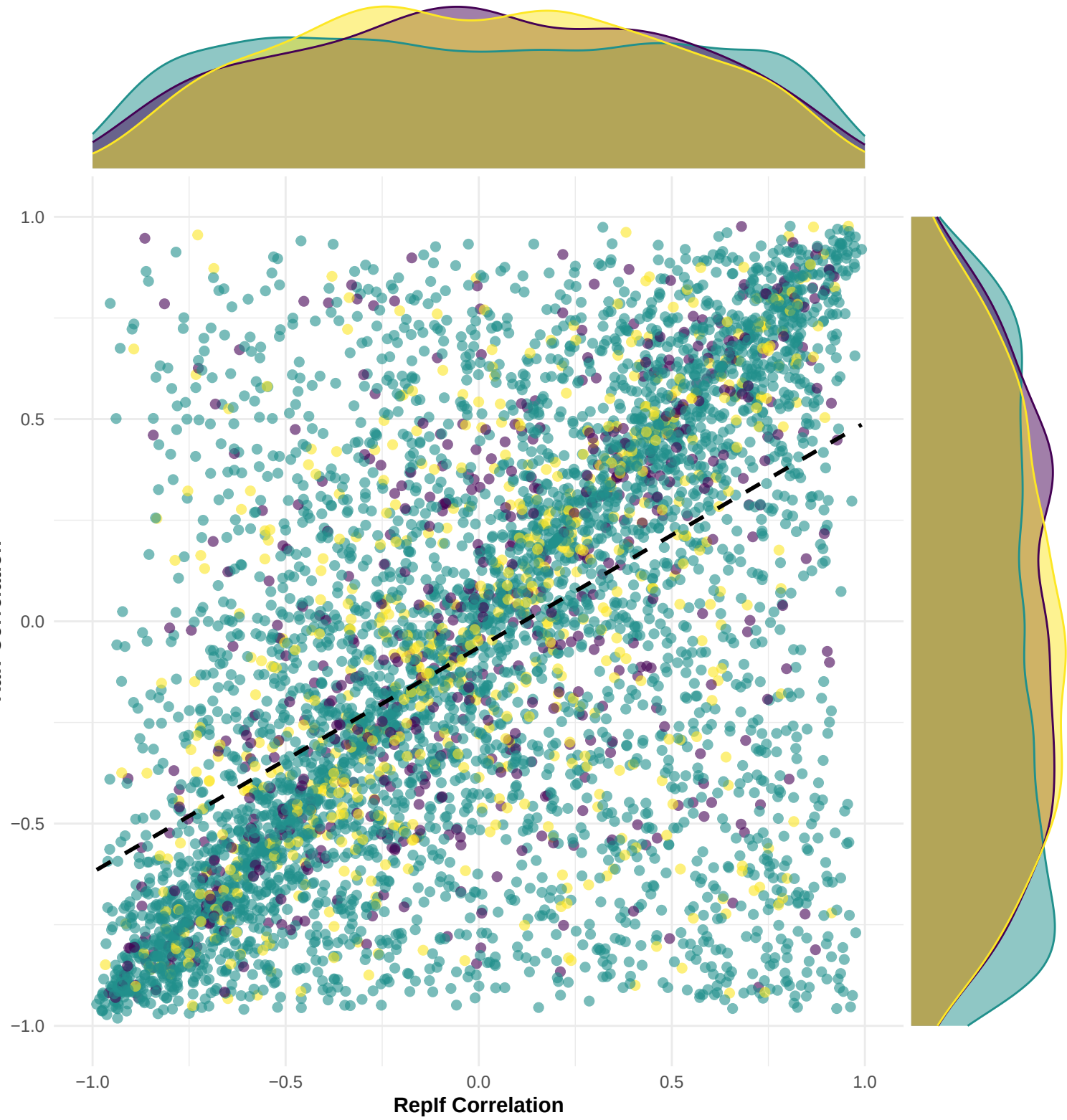
ForeBrain – Methylation–Expression Correlations
