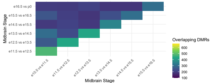
DMR Persistence Across Consecutive Stages
