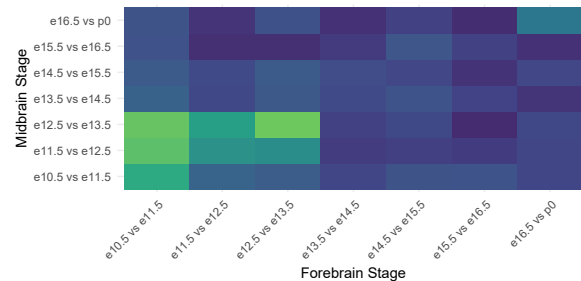
Cross-tissue DMR Overlaps
