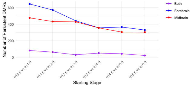
DMR Persistence Across Consecutive Stages
