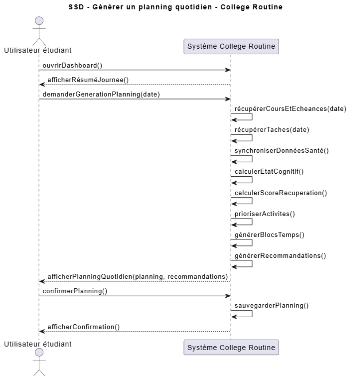
FIGURE 3 – SSD - Générer un planning quotidien - College Routine
