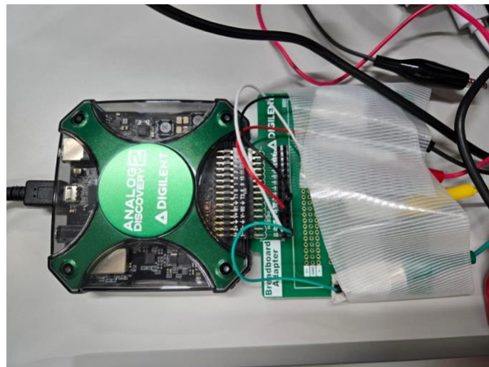
図 8 Analog Discovery2 (DIGILENT 社)
