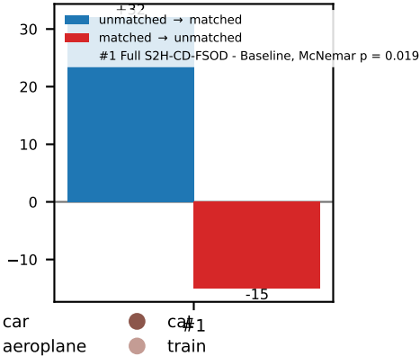
match-status flips, same queries
