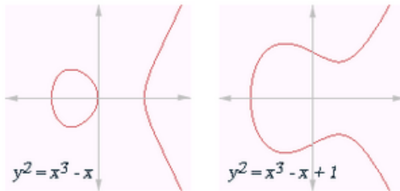
Gambar 22: Contoh-contoh kurva eliptik real
