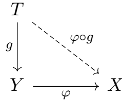
Figure 1: The map \varphi(T) : Y(T) \rightarrow X(T) .
