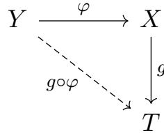
Figure 2: The map T(\varphi) : T(X) \rightarrow T(Y) .
