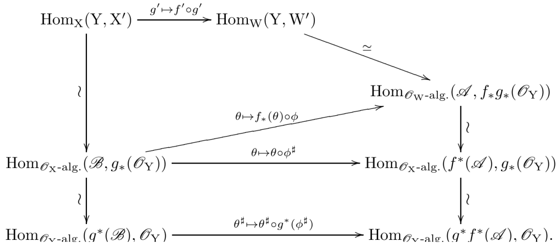
Figure 61: Functoriality of the affine-scheme/algebra correspondences.
