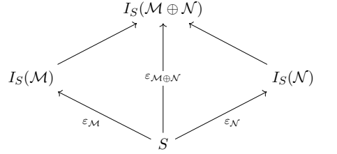
Figure 5: The induced commutative diagram of S -schemes.
