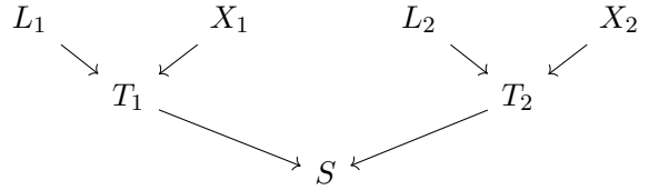
Figure 57: The objects L_i, X_i over T_i , and T_i over S .
