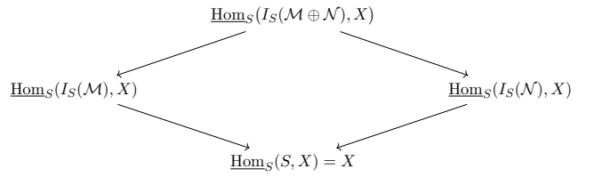
Figure 6: The cartesian diagram of \underline{\mathrm{Hom}}_S -functors.
