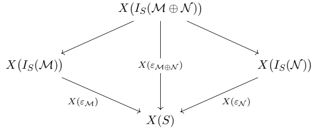
Figure 7: The cartesian diagram after evaluation on S .
