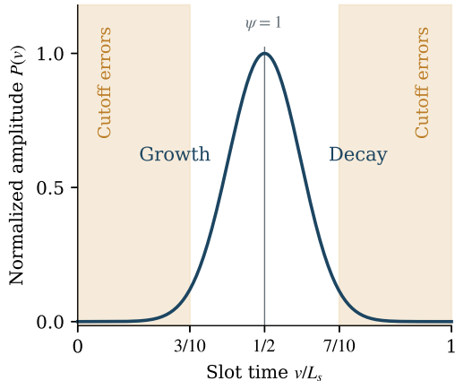
(b) Growth followed by viscous decay
