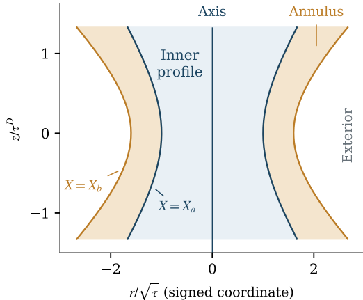
(a) The radial regions at fixed time
