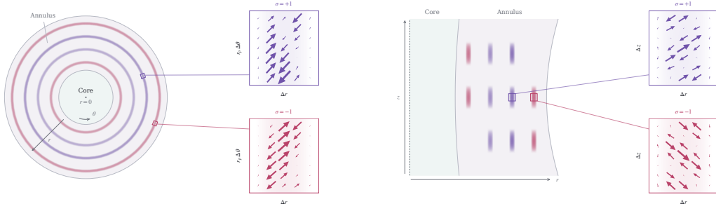
Figure 2: Pulse geometry and perturbation velocities. Left : At fixed height, pulse envelopes occupy complete rings; the close-ups show radial and azimuthal perturbation velocities. Right : A radial-axial section, where each localized patch is a cross-section of a complete ring; the close-ups show radial and axial perturbation velocities. Colors distinguish the two families. The specific pulse arrangement shown is schematic; active locations, spacing, and aspect ratios are illustrative.
