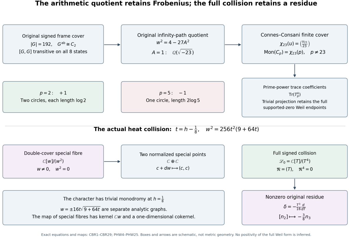
Figure 11: The original frame-cover quotient, its arithmetic specialization and prime returns, the two different special-fibre maps, and the surviving holonomy residue. CBR1-CBR29 and PHW4-PHW25 prove these exact maps. The box arrangement is schematic.
