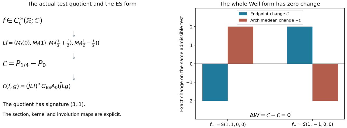
Figure 6: The actual four-value correction, its exact ES isometry, and its cancellation in the full Weil form. WEC1–WEC18 give all maps, the section and the two admissible tests.
