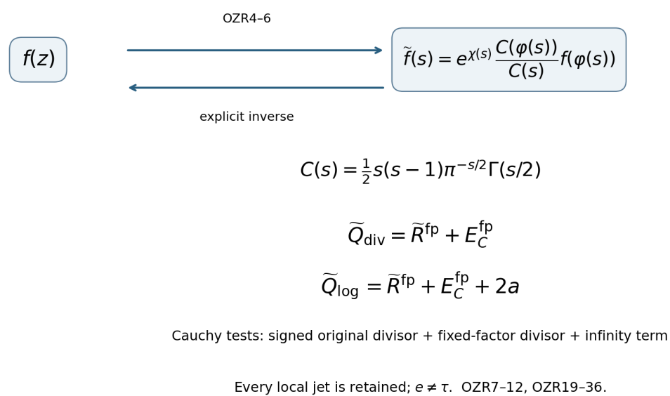
Figure 27: The complete original-zeta map and the exact inverse in OZR4–6 preserve every exceptional valuation and jet by OZR7–12. Here \chi(s)=a(s-1/2)^2+ib(s-1/2)+c . For the Cauchy test the complete signed-divisor trace, fixed-factor trace, and infinity contribution are the three separately retained quantities in OZR19–36. The plus 2a term belongs to the logarithmic kernel. OZR33 proves its full negative-index effect.
