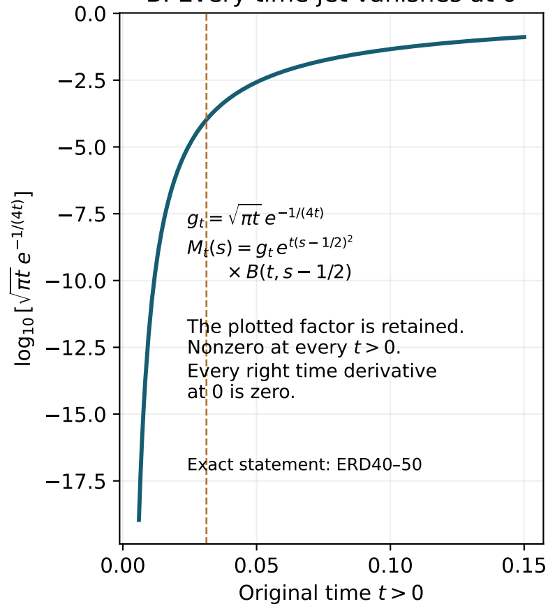
B. Every time jet vanishes at 0
