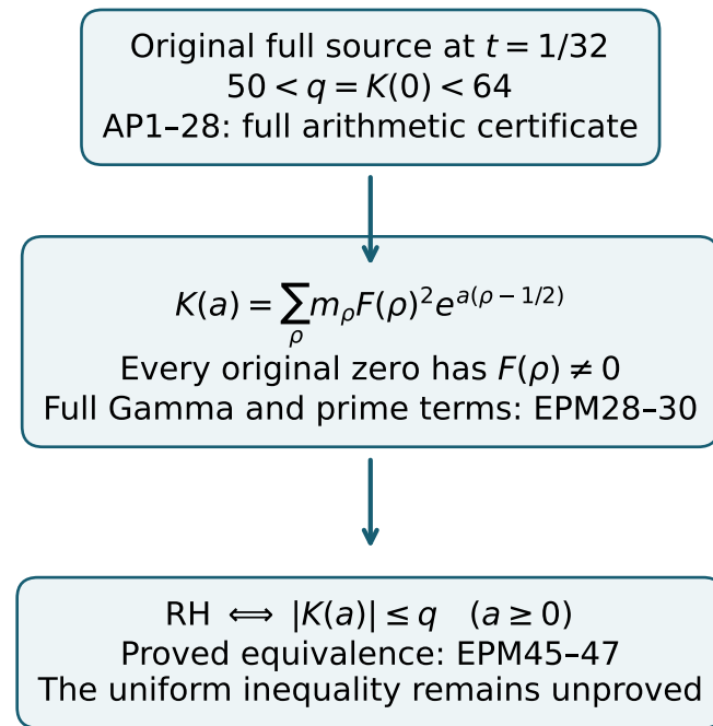
C. The positive test and the remaining bound
