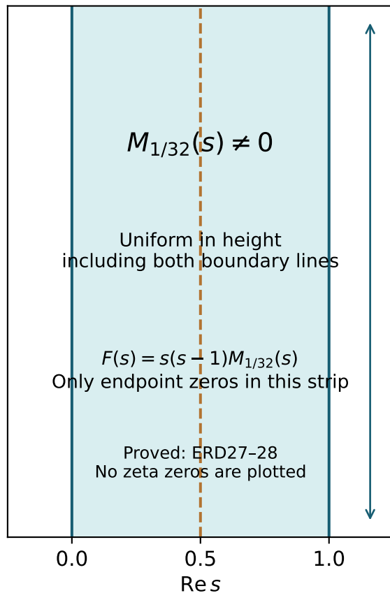
A. No missing zero in the strip
