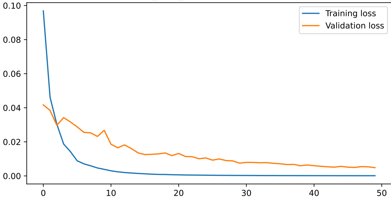
arima_lstm_hybrid Training History
