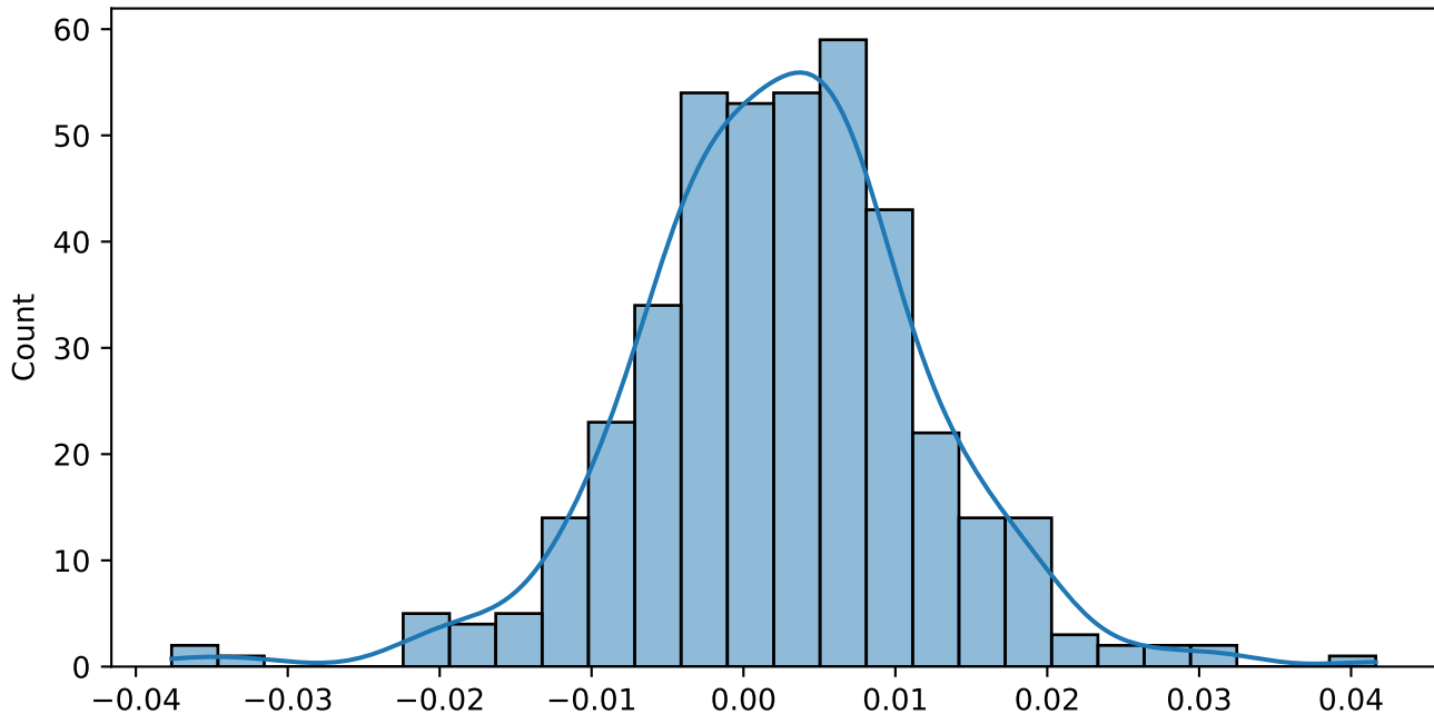
linear_regression Residual Distribution
