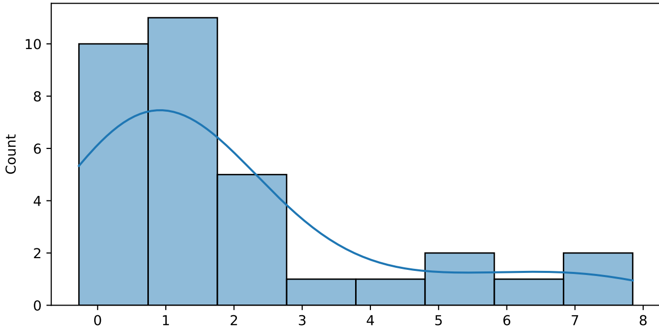
Istm Residual Distribution
