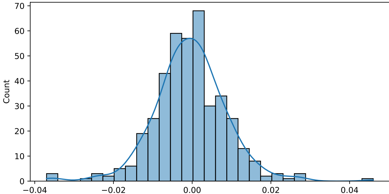
persistence Residual Distribution
