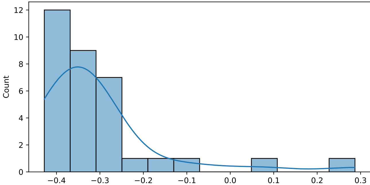
transformer Residual Distribution
