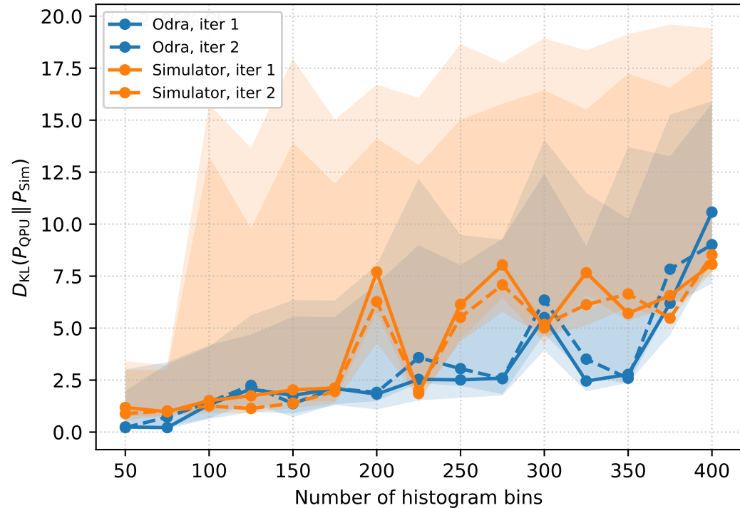
QPU vs Sim
