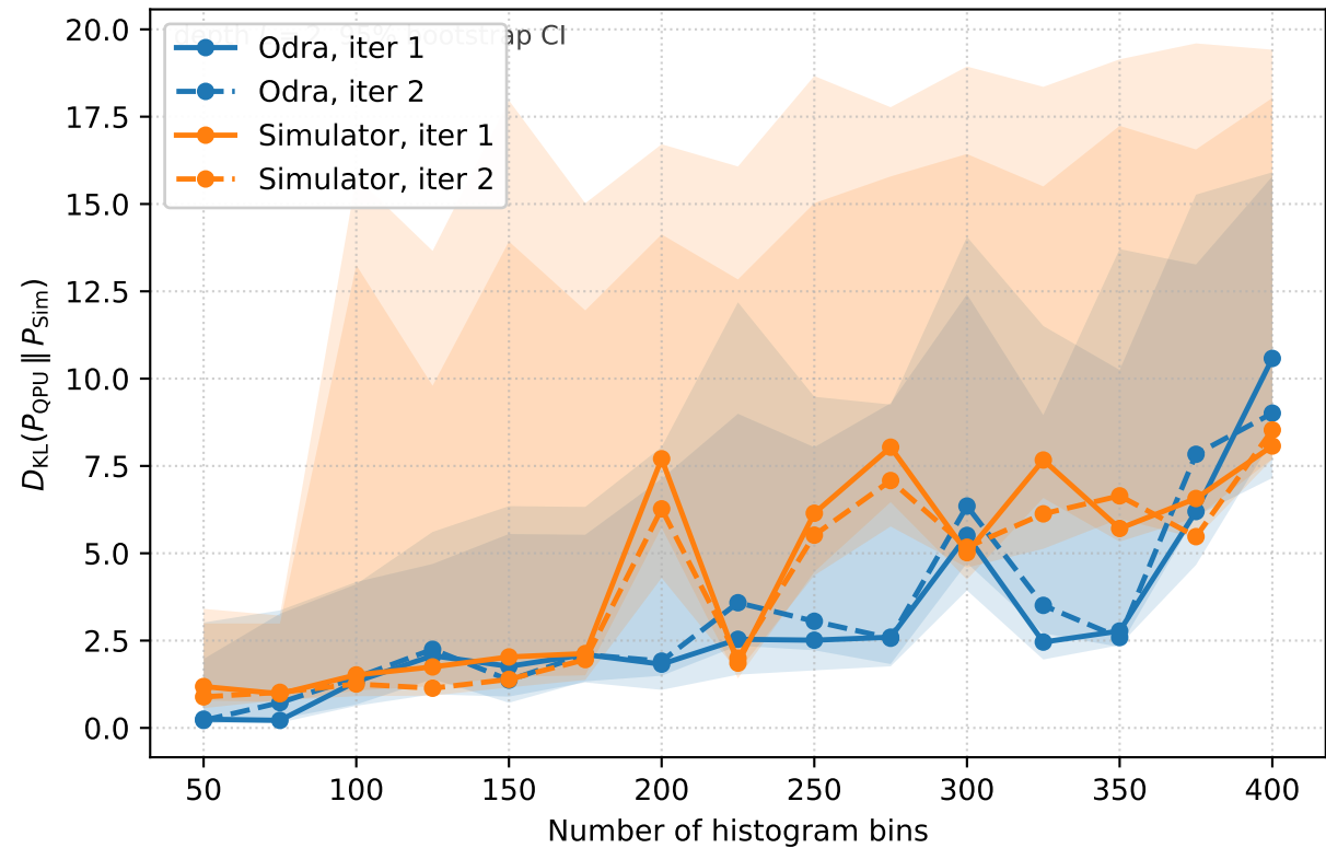
Odra vs Simulator: QPU vs Sim
