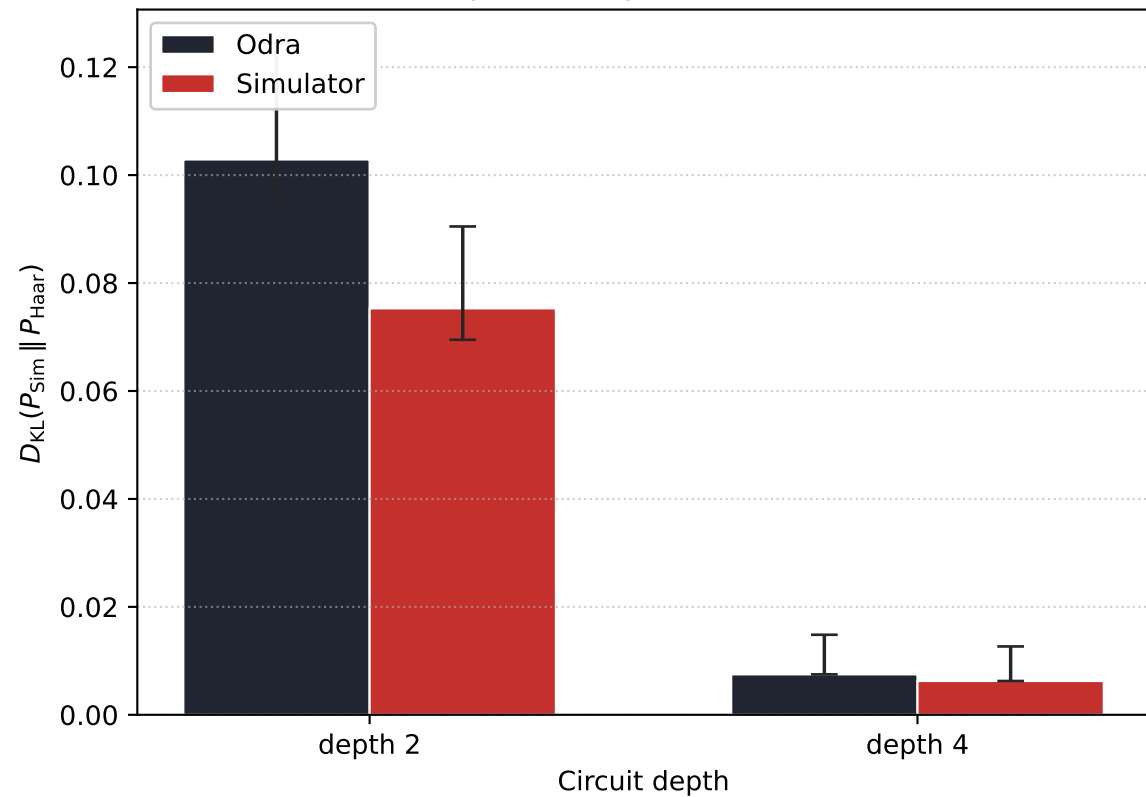
Expressibility on Simulator
