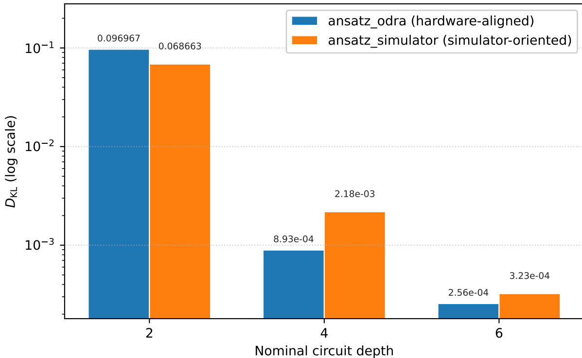
D_{\text{KL}}(p_{\text{emp}} \parallel q_{\text{Haar}}) vs. nominal depth
